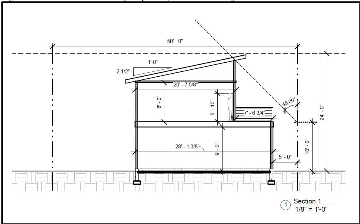
Figure 2: Side Yard Second Story Step Back, 2-Foot Eave Projection Allowed
