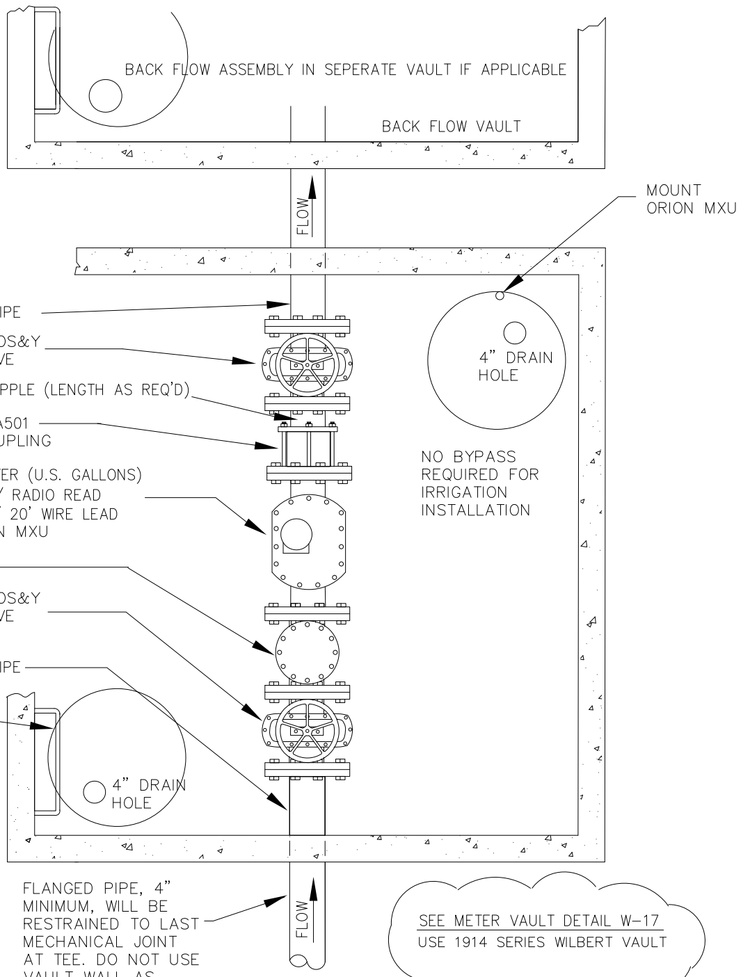
PLAN VIEW
